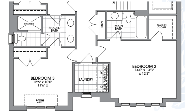
SECOND FLOOR ELEVATION B & C
