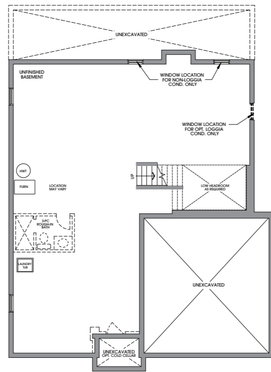
BASEMENT ELEVATION A
