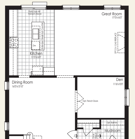
Opt. Ground Floor Part. Elevation A
