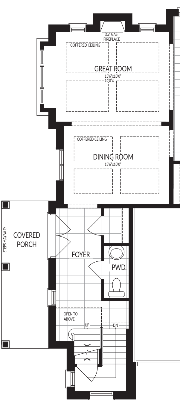
GROUND FLOOR PLAN, STYLE 'B'
