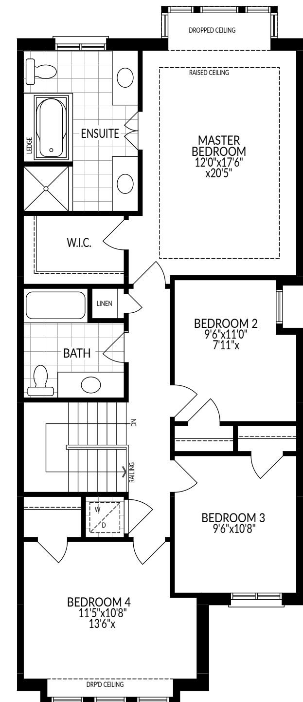
OPT. SECOND FLOOR PLAN STYLE 'A' (4 BEDROOM PLAN) ('B' & 'C' SIMILAR)
