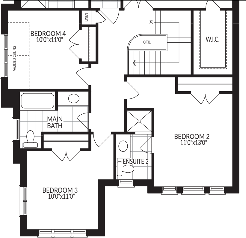
SECOND FLOOR PLAN STYLE 'B'
