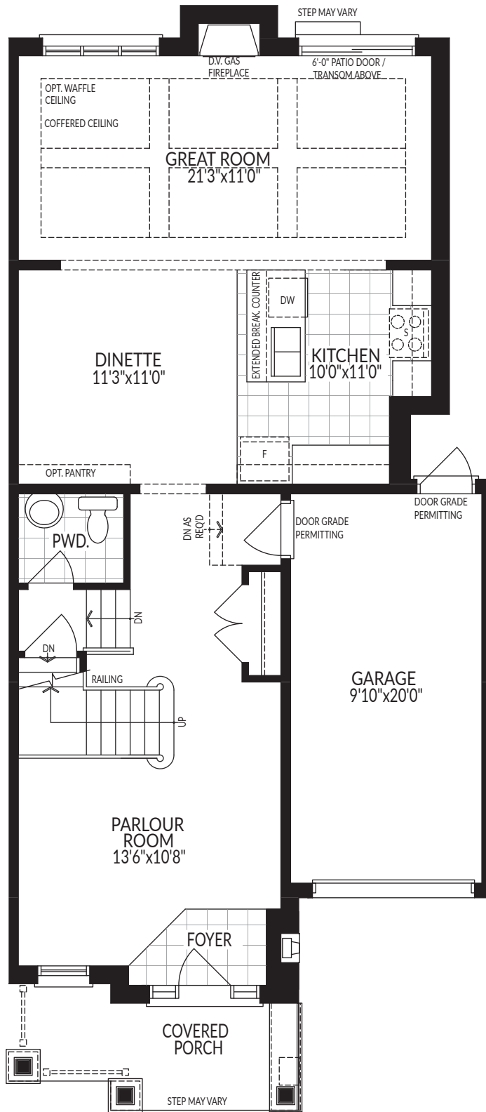
GROUND FLOOR PLAN STYLE 'A'
