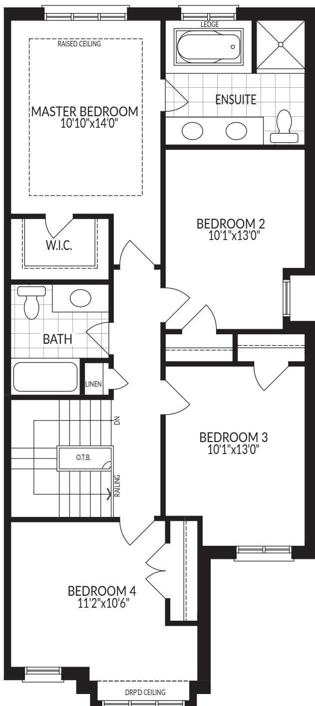
OPT. SECOND FLOOR PLAN STYLE 'A' (4 BEDROOM PLAN) ('B' & 'C' SIMILAR)
