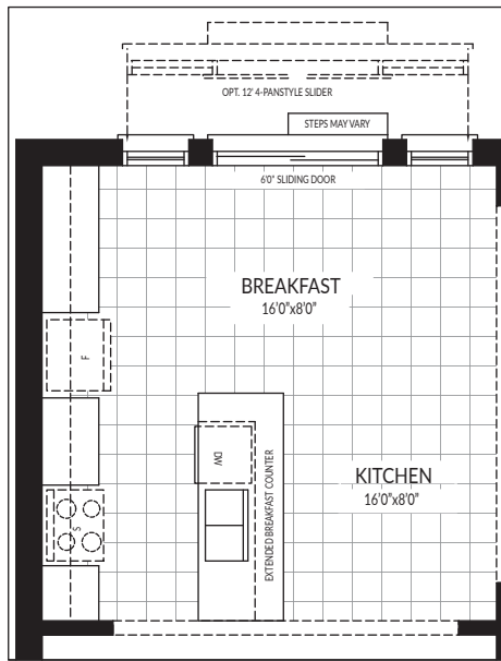
OPT. KITCHEN / BREAKFAST LAYOUT
