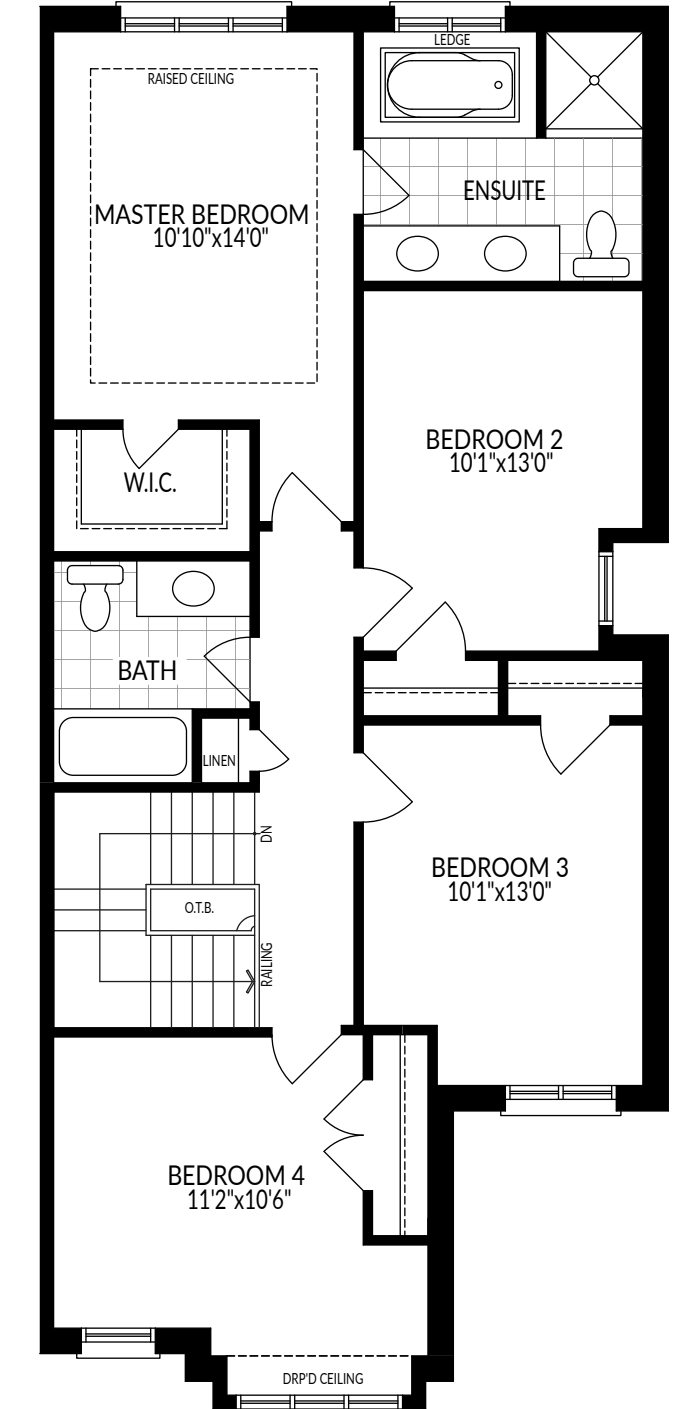
OPT. SECOND FLOOR PLAN STYLE 'A' (4 BEDROOM PLAN) ('B' & 'C' SIMILAR)
