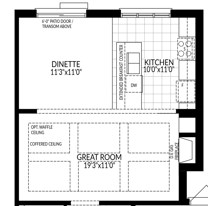
PARTIAL OPT. GROUND FLOOR PLAN STYLE 'A', 'B' & 'C'
