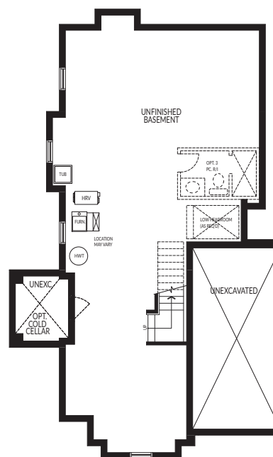
BASEMENT PLAN, STYLE 'A'
