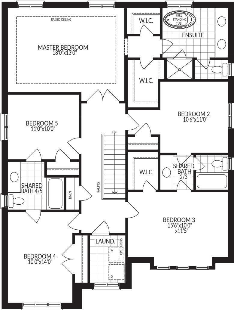
OPT. SECOND FLOOR PLAN, STYLE 'A' - 5 BEDROOM LAYOUT (STYLE 'B' & 'C' SIMILAR)
