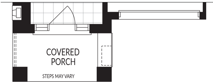
GROUND FLOOR PLAN, STYLE 'C'
