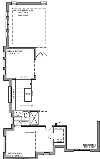
PARTIAL SECOND FLOOR ELEVATION B
