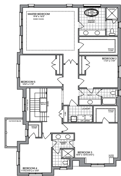
OPT. SECOND FLOOR WITH 5 BEDROOM ELEVATION A
