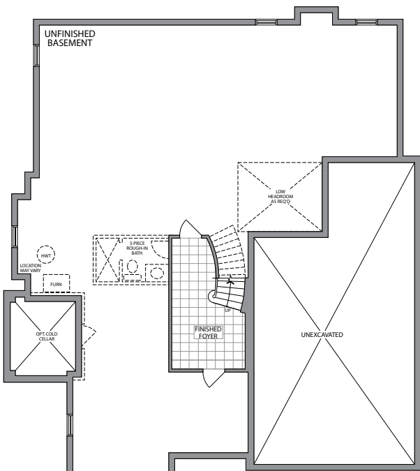
BASEMENT ELEVATION A
