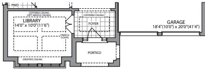
GROUND FLOOR ELEVATION B
