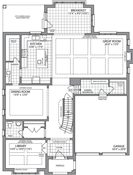
OPTIONAL GROUND FLOOR ELEVATION A (ELEVATION B SIMILAR)
