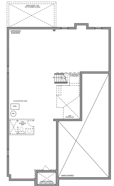
BASEMENT PLAN, ELEV. 'A'
