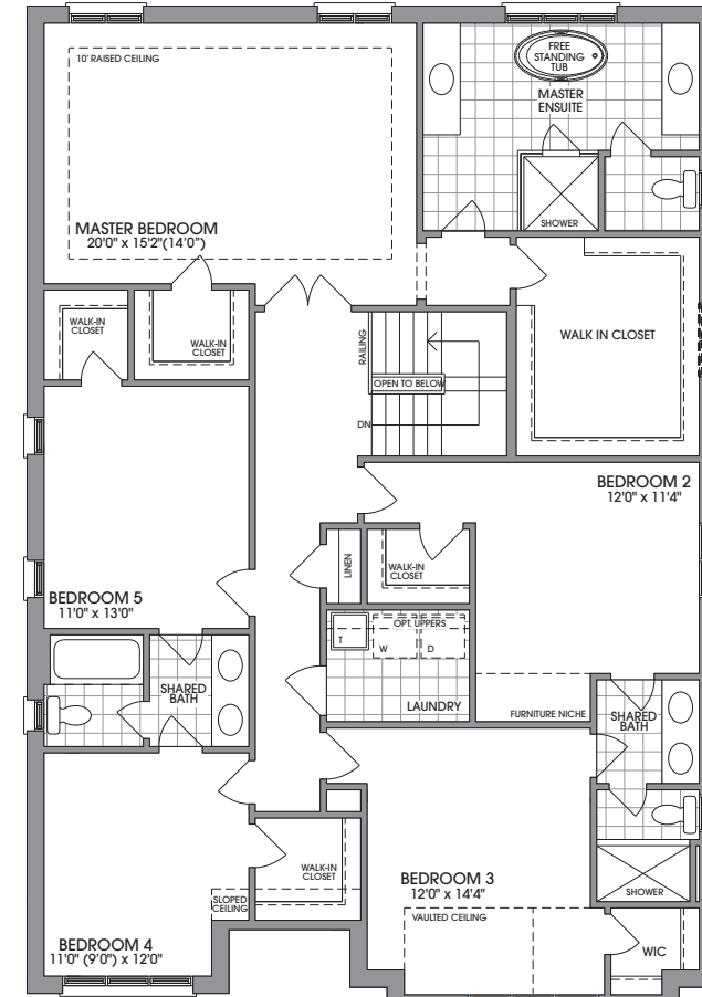
OPTIONAL 5 BEDROOM SECOND FLOOR PLAN, ELEV. 'A'
