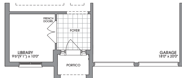
GROUND PLAN, ELEV. 'B' & 'C'
