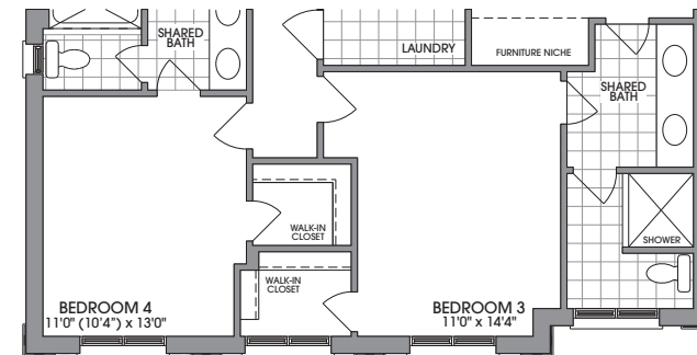
OPTIONAL 5 BEDROOM SECOND FLOOR PLAN, ELEV. 'B' & 'C'
