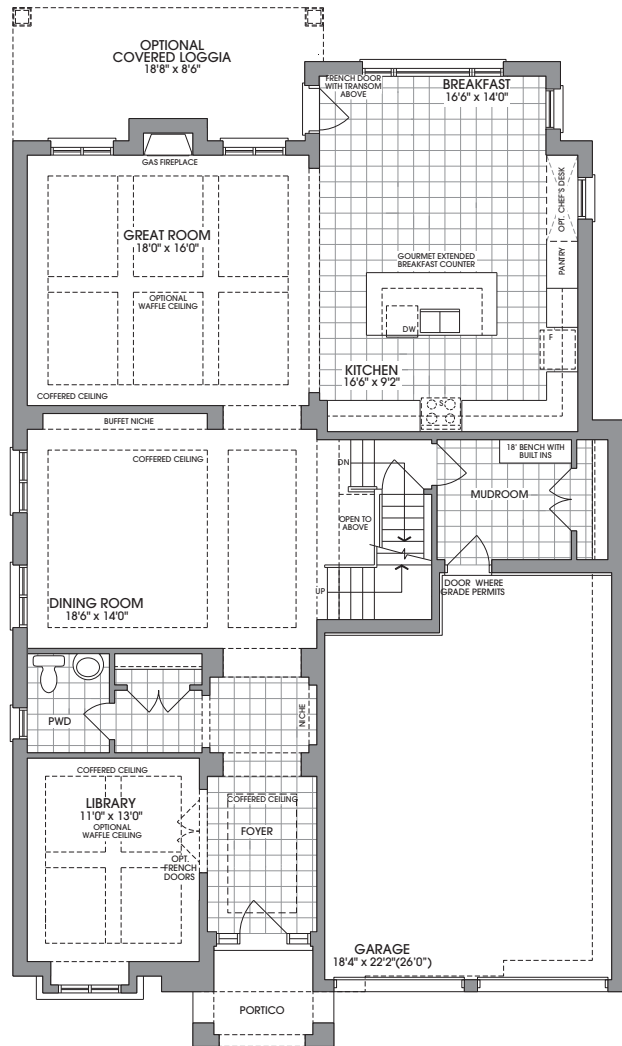
GROUND PLAN, ELEV. 'A'
