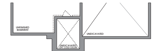
BASEMENT PLAN, ELEV. 'B' & 'C'
