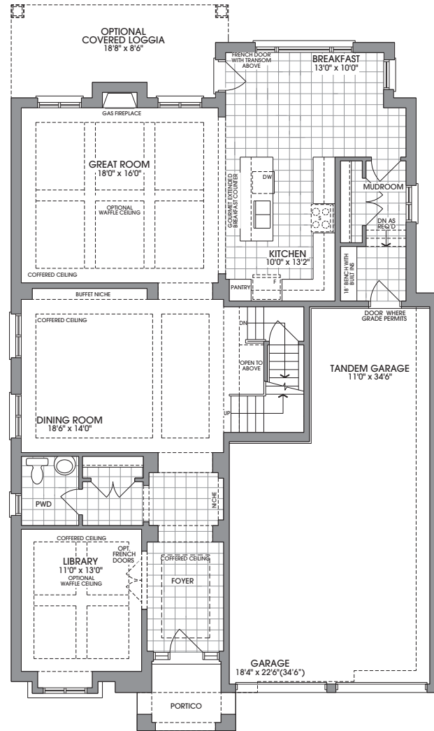
OPTIONAL GROUND PLAN WITH TANDEM GARAGE
